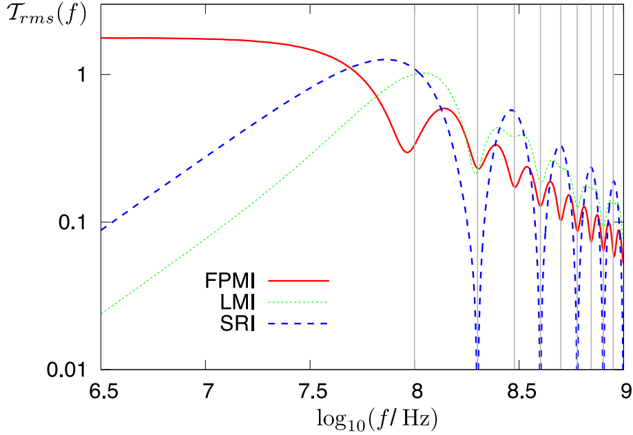
Figure 6.5: GW response function \mathcal{T}_{\text{rms}}(f) . Vertical lines are plotted at multiples of 100 MHz.
