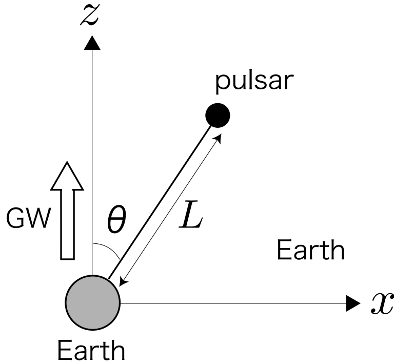
Figure 4.1: Doppler tracking.
