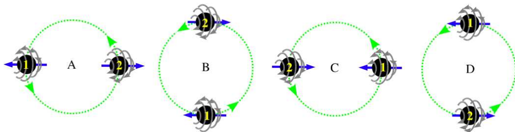
Figure 13.3: Pretorius' Explanation
