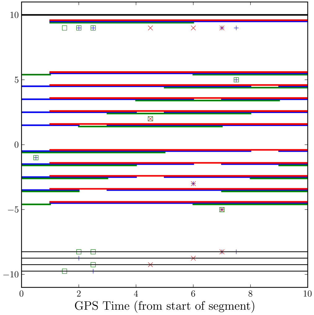
Figure 8.2: SEPTIME Example
