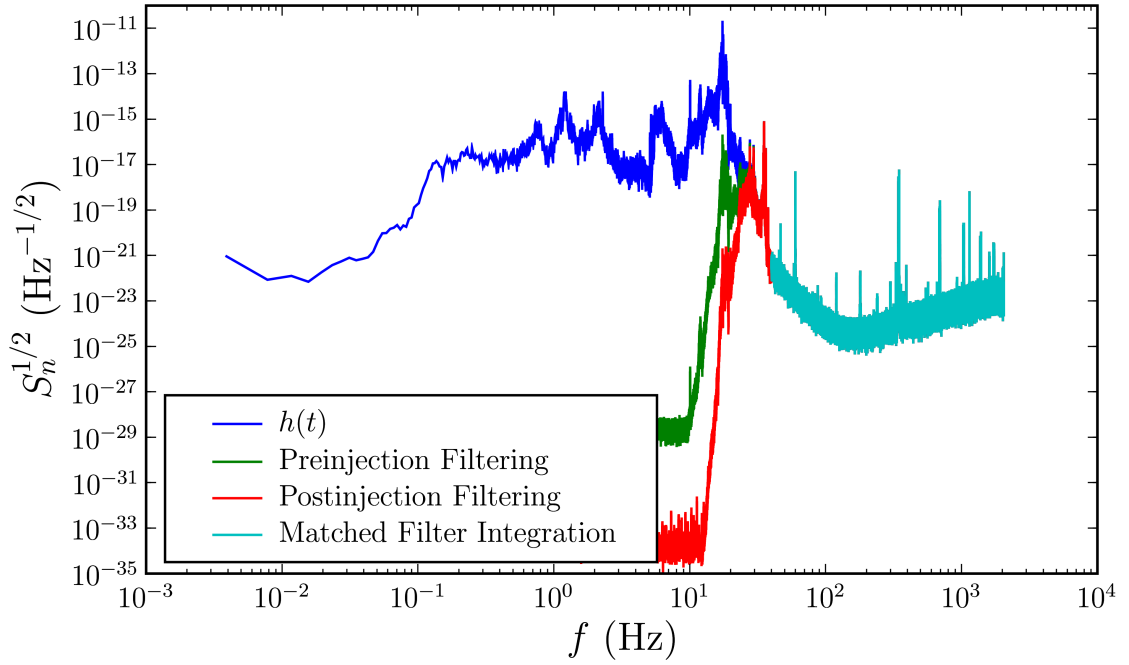
Figure 6.2: Data Preprocessing
