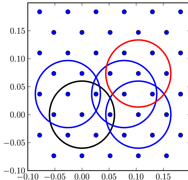
Figure 6.4: Trigscan Example
