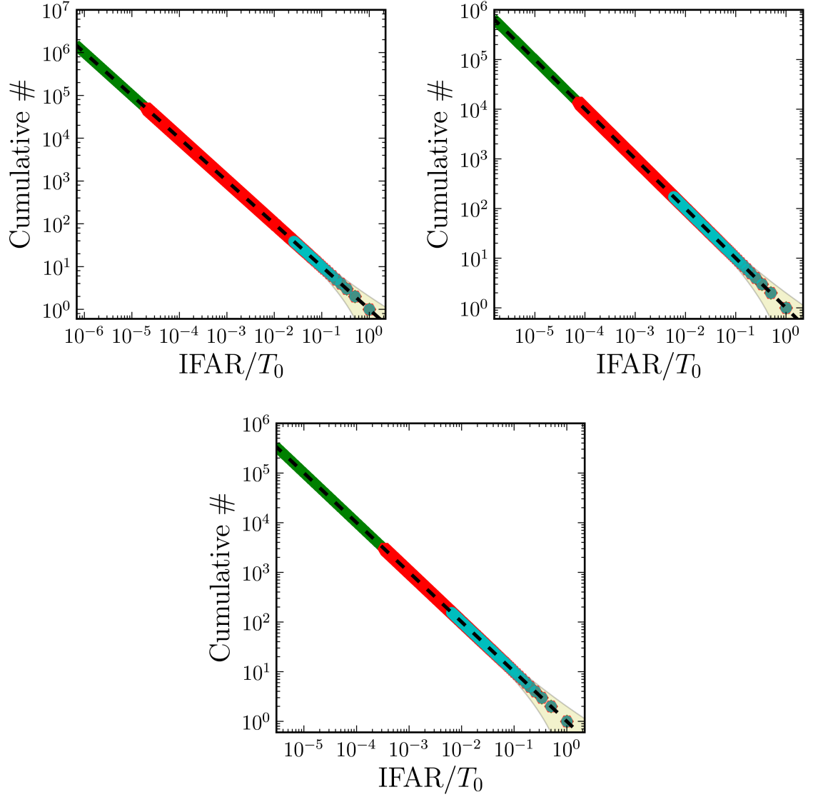
Figure 7.6: Background IFAR Plots
