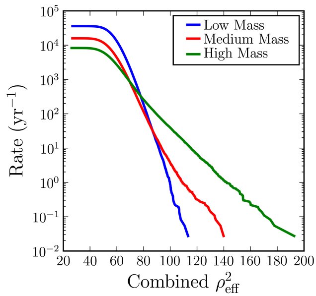
Figure 7.5: Combined \rho_{\text{eff}}^2 Distributions for Background Triggers for Different Chirp Mass Bins
