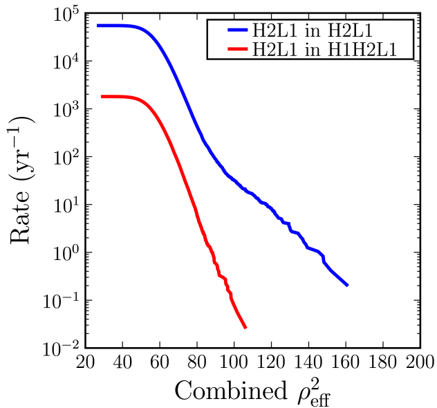
Figure 7.2: Effect of Amplitude Veto on Background Trigger Rate
